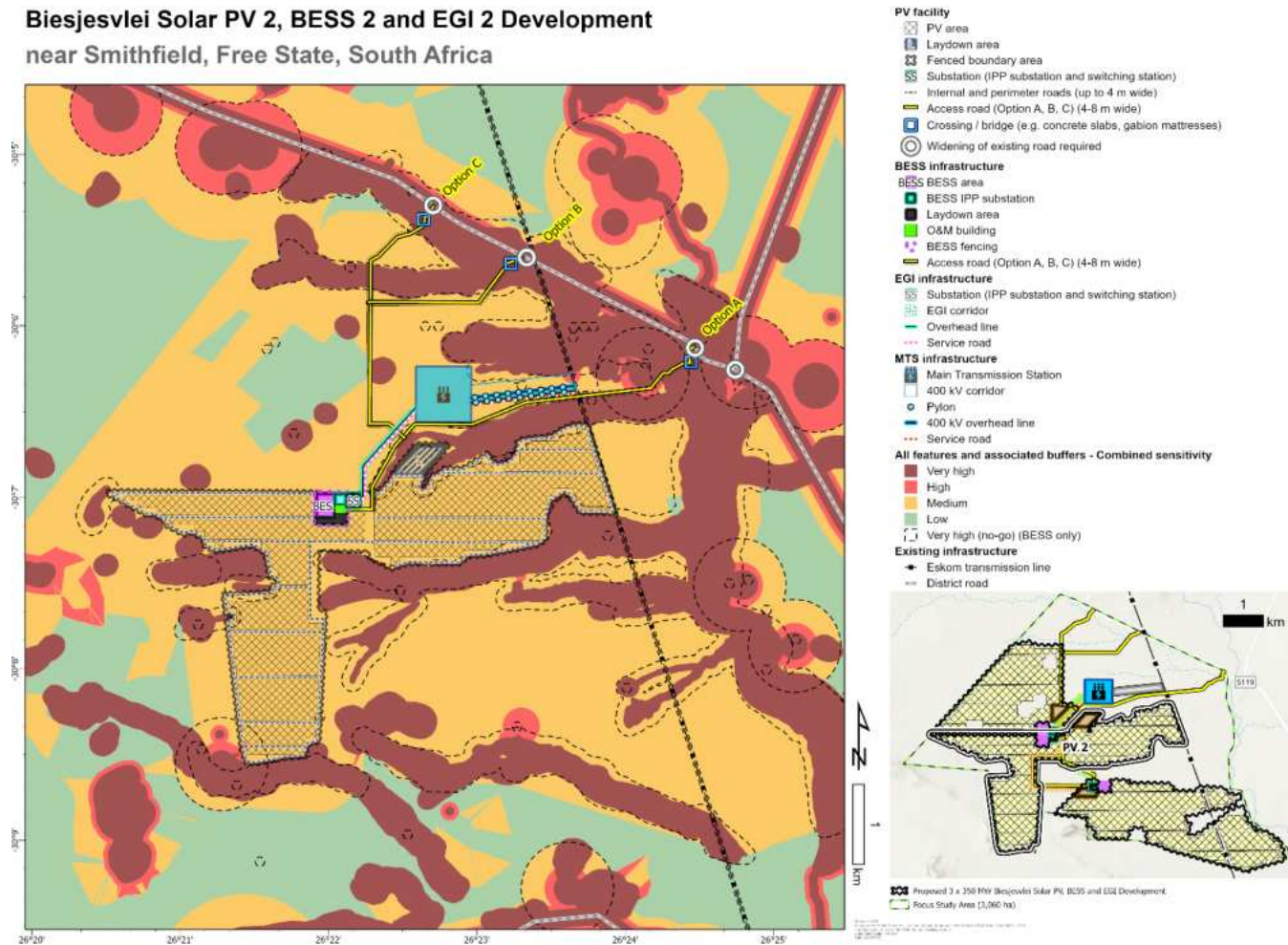
Figure 20.8: Combined Final Project Layout and Sensitivity Map for Project 2 (Biesjesvlei PV2), Project 5 (Biesjesvlei BESS 2), and Project 8 (Biesjesvlei EGI 2) [including Project 10 (Biesjesvlei MTS and LILO).
