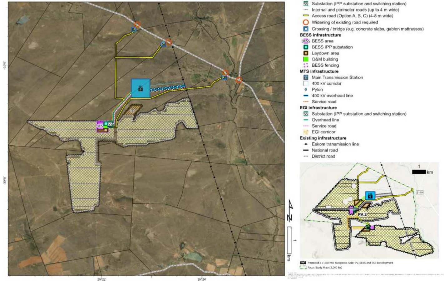
Figure 20.4: Final Project Layout for Project 2 (Biesjesvlei PV2), Project 5 (Biesjesvlei BESS 2), and Project 8 (Biesjesvlei EGI 2) [including Project 10 (Biesjesvlei MTS and LILO)].
