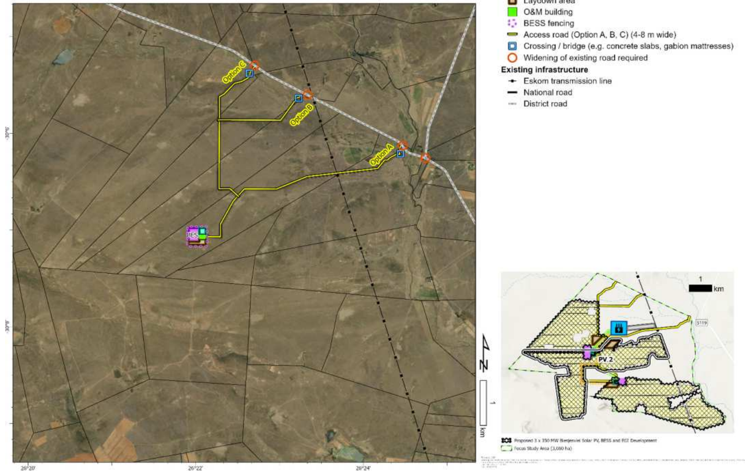
Figure 20.2: Final Project Layout Map showing the detailed infrastructure and development footprints for Biesjesvlei BESS 2.
