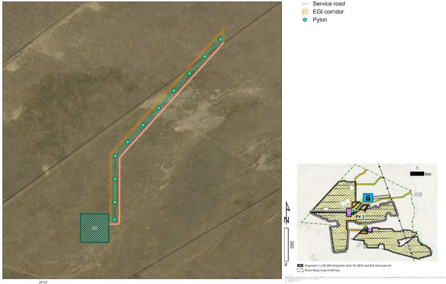
Figure 20.3: Final Project Layout Map showing the detailed infrastructure and development footprints for Biesjesvlei EGI 2.
