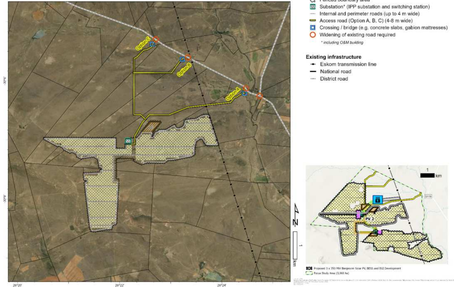
Figure 20.1: Final Project Layout Map showing the detailed infrastructure and development footprints for Biesjesvlei PV2.
