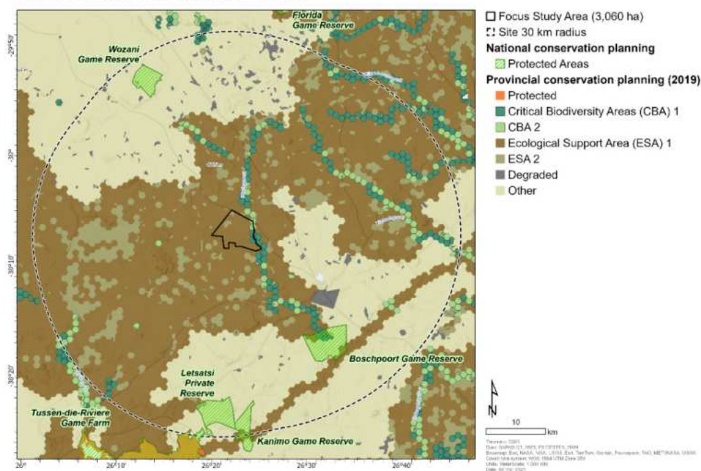
Figure 3.20: Provincial Conservation Planning within the study area based on the 2019 FSPBP, and National Conservation Planning in terms of the South African Protected Areas Database (SAPAD; Quarter 1, 2024).
