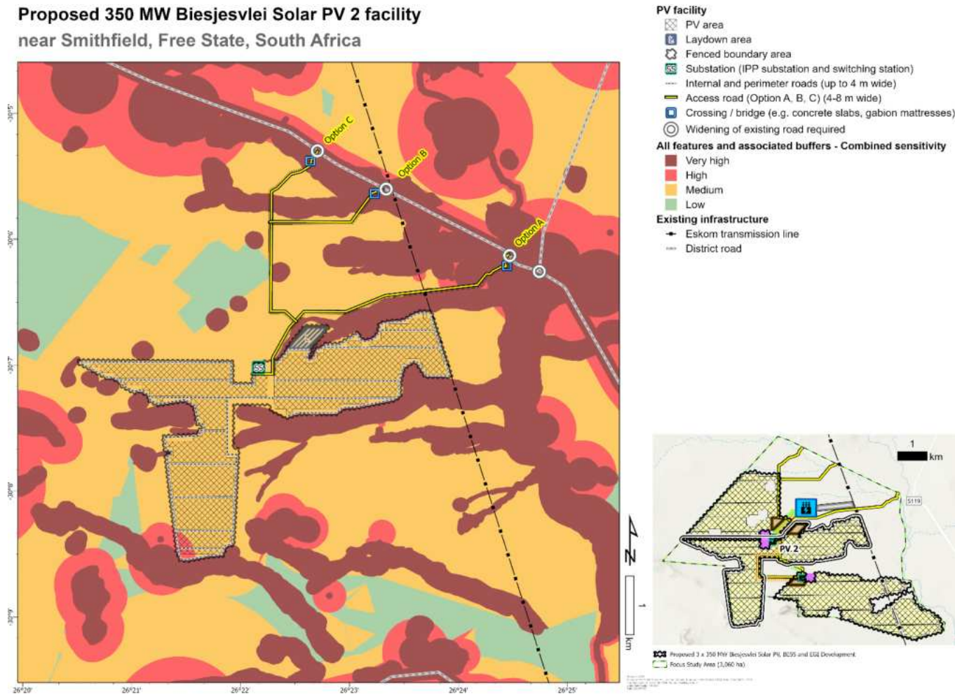
Figure 20.5: Combined Final Project Layout and Sensitivity Map for Biesjesvlei PV2.
