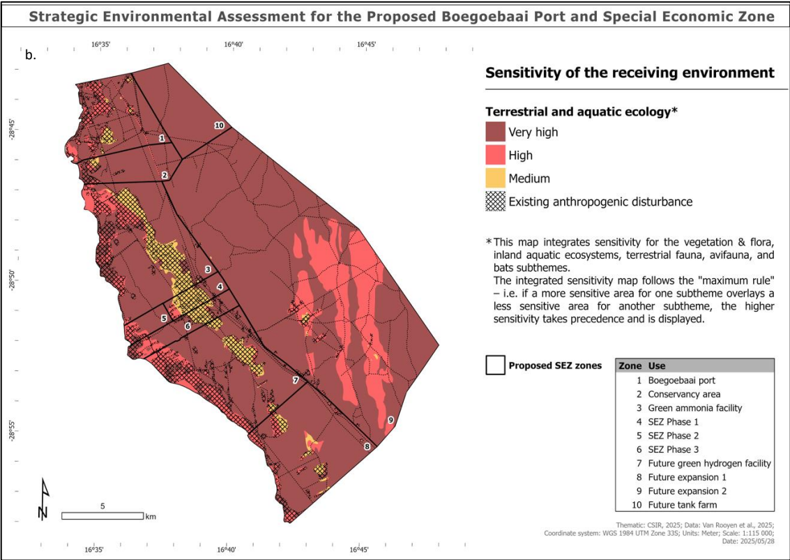
Figure 3-26: (a) & (b) Integrated site sensitivity of the Aquatic and Terrestrial Ecology studies of the Boegoebaai Port and SEZ.
