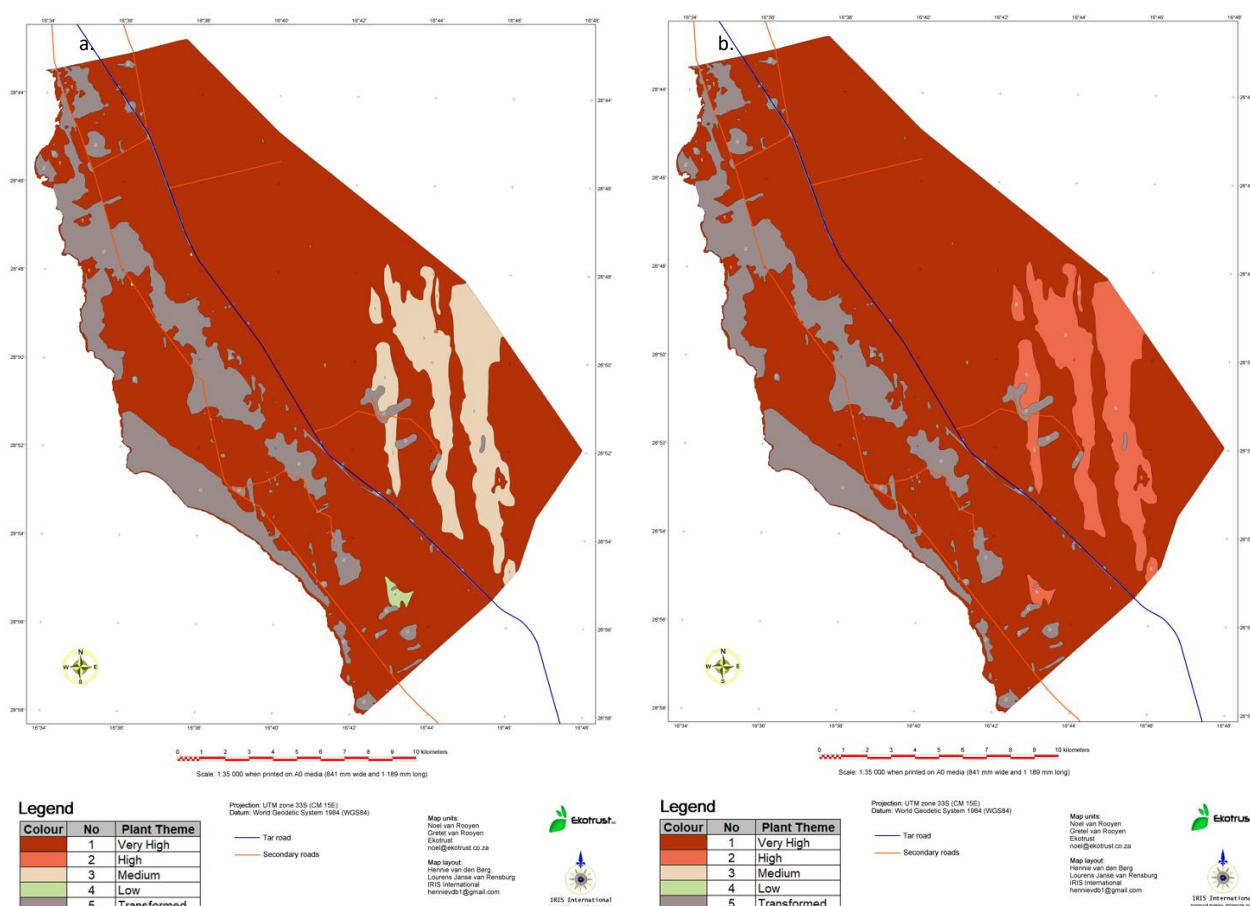
Figure 3-25: Site sensitivity of (a) the Plant Theme and (b) the Relative Terrestrial Biodiversity Theme for the Boegoebaai Port and SEZ site as found in the current study.
