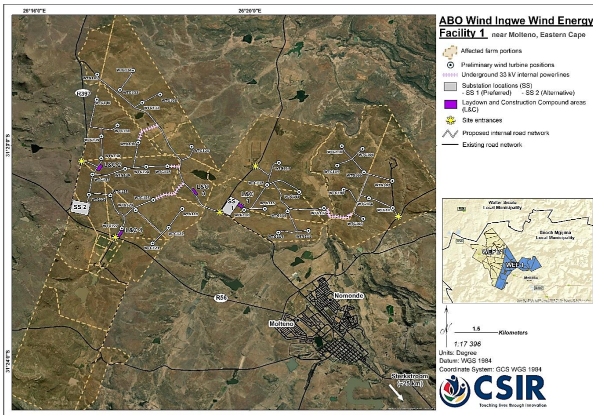
Figure B. Indicative site layout plan of the proposed Ingwe WEF 1 as assessed during the Scoping phase.
