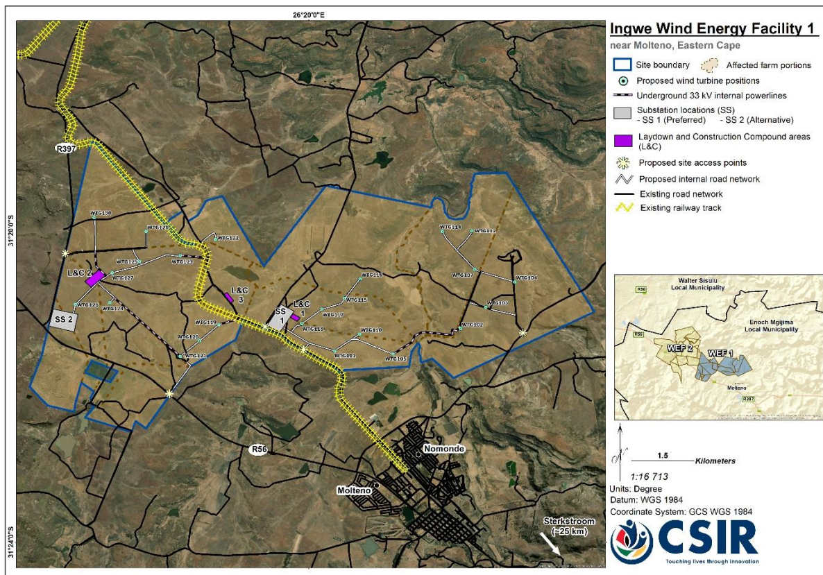
Figure C. The current reduced site layout plan of the proposed Ingwe WEF 1 as assessed during the EIA phase.
