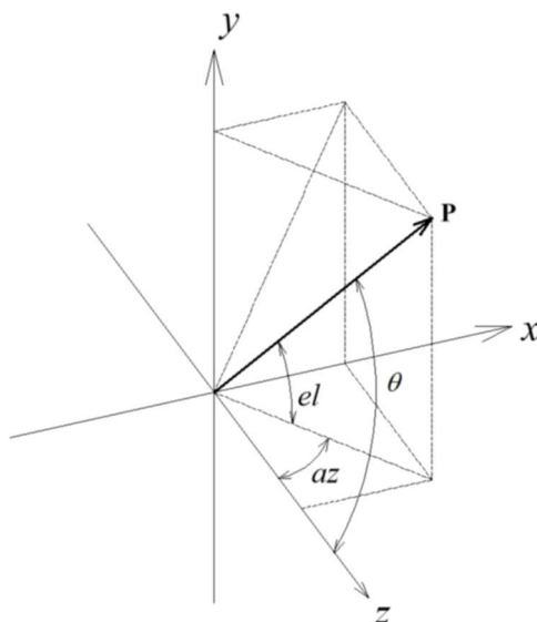
Figure 2: Coordinate system employed to define the antenna direction.
