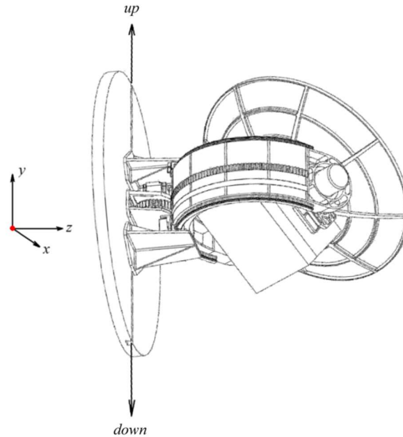
Figure 3: A vertically mounted Azimuth-Elevation antenna positioner similar to that which could be employed in the Inundu pod.
