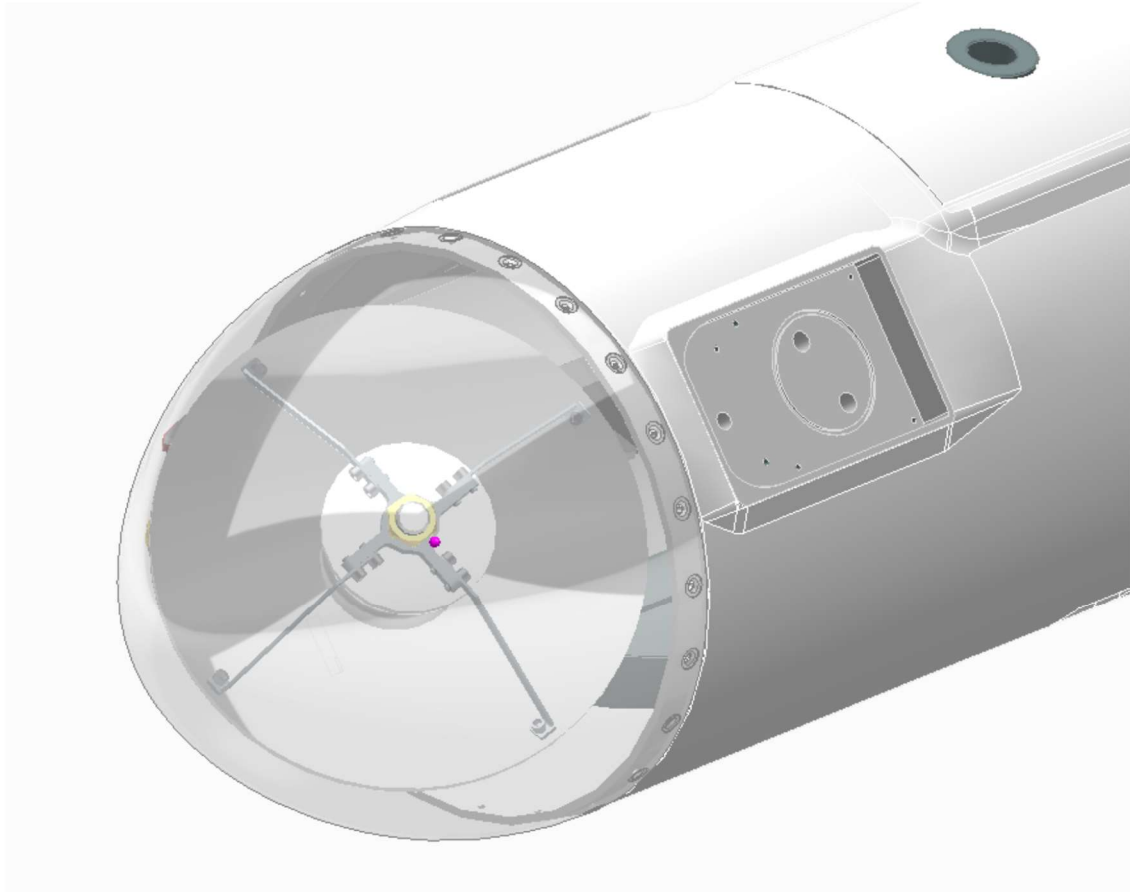
Figure 4: Azimuth-Elevation antenna positioner concept adjusted to az=45^\circ and el=45^\circ , viewed through a transparent nosecone from in front while installed in Inundu POD.
