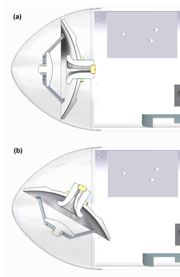
Figure 1: The Cassegrain MW Antenna located within the nosecone of the Inundu-3 airborne pod.
