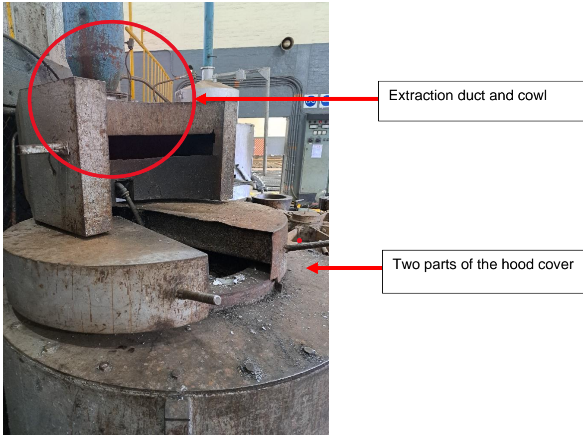
Fig 3A: Extraction duct and hood in a partially open position
