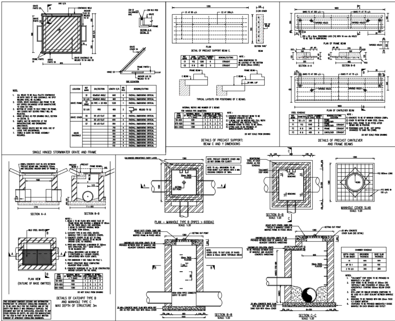
Figure 6: Stormwater details: manhole and inlet plans.
