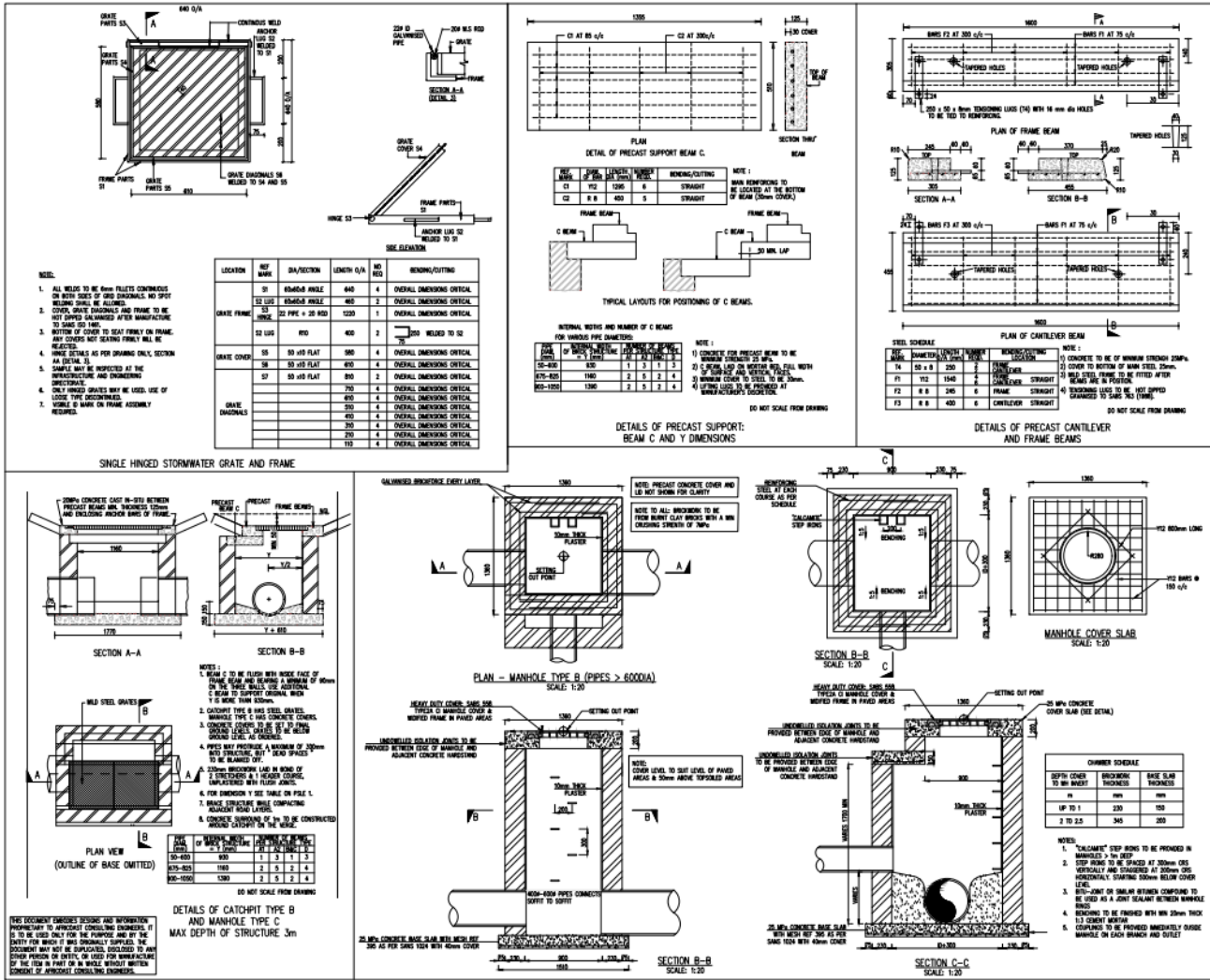
Figure 5: Stormwater details: manhole and inlet plans.
