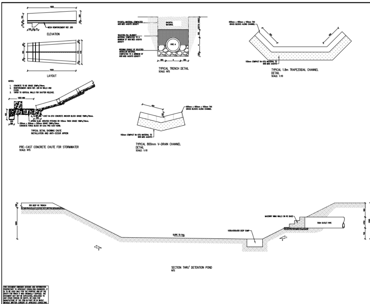
Figure 4: Stormwater details: trench, chute, and channels plan.
